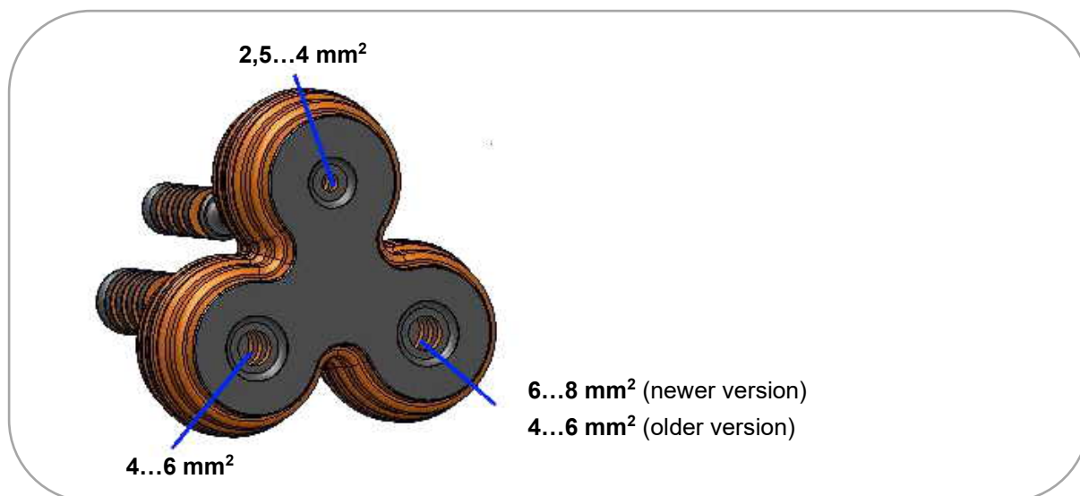
Fig. 48: Service slot cover IP69K
