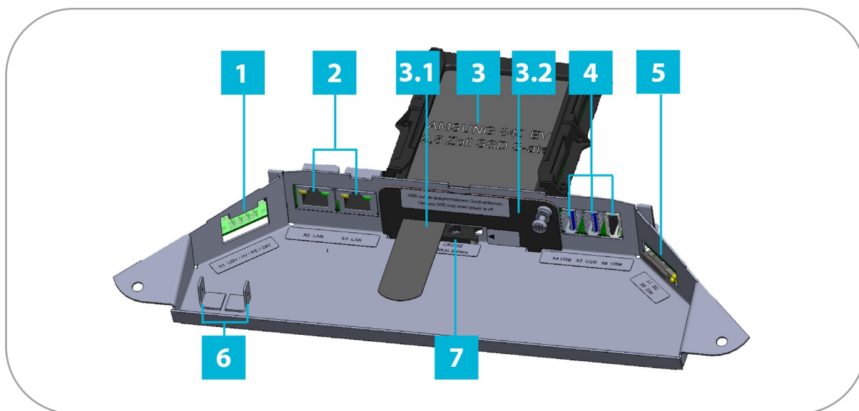
Figure 9: Service slot – MMT 8000 series
