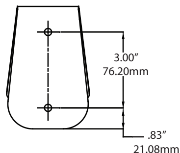
WALL MOUNTING
