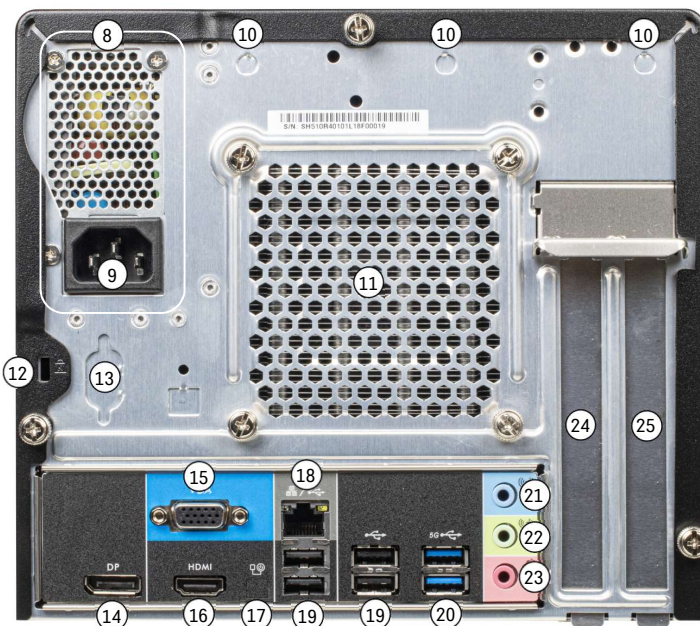
Back panel
