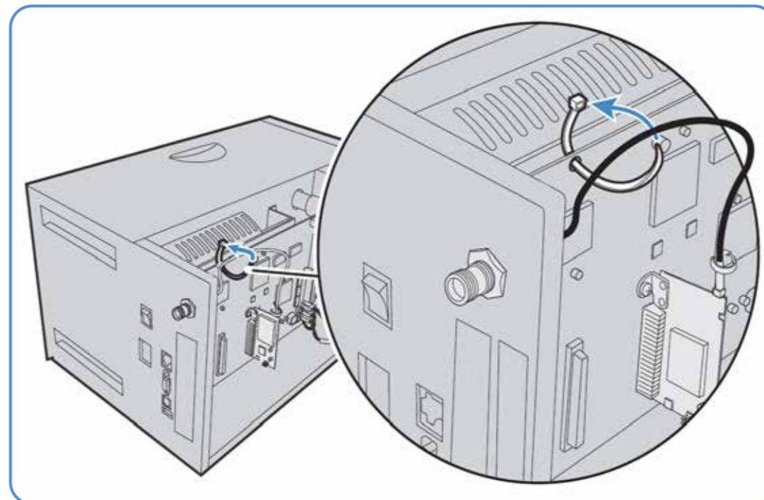
Route antenna cable to back plate
