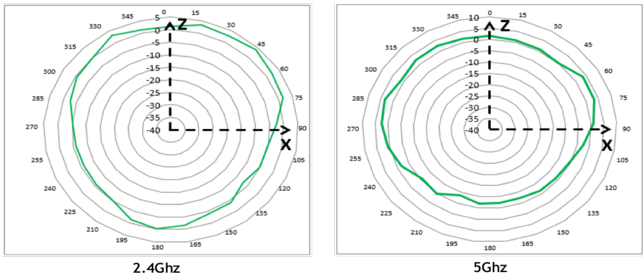
Figure 1. OmniAccess AP1321 antenna pattern plots
