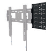
AWL05-750BL AV hardware rack Capacity: 10 kg For Apple-TV, mini-PC, NUC and more Suitable as backplate connector for multiple screen setup
