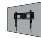
WL30-750BL16 Screen size: 42-86" Capacity: 125 kg VESA: 100x100 - 600x400
