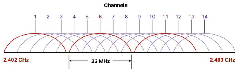
Figure 9. IEEE 802.11b/g DSSS Channel Allocations
