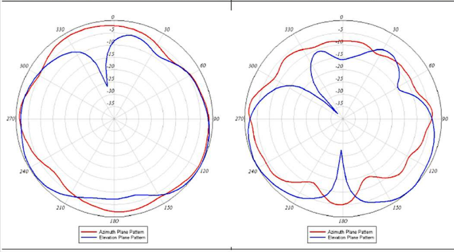
2.4-GHz Element 2 Azimuth and Elevation Plane Patterns 5-GHz Element 2 Azimuth and Elevation Plane Patterns
