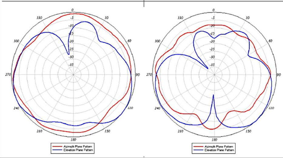
2.4-GHz Element 1 Azimuth and Elevation Plane Patterns 5-GHz Element 1 Azimuth and Elevation Plane Patterns
