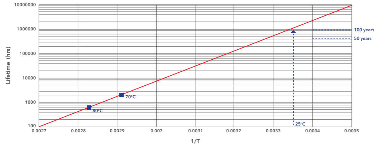
Life Estimation of MKM DVD+RDL (Life End: PI Error =280)
