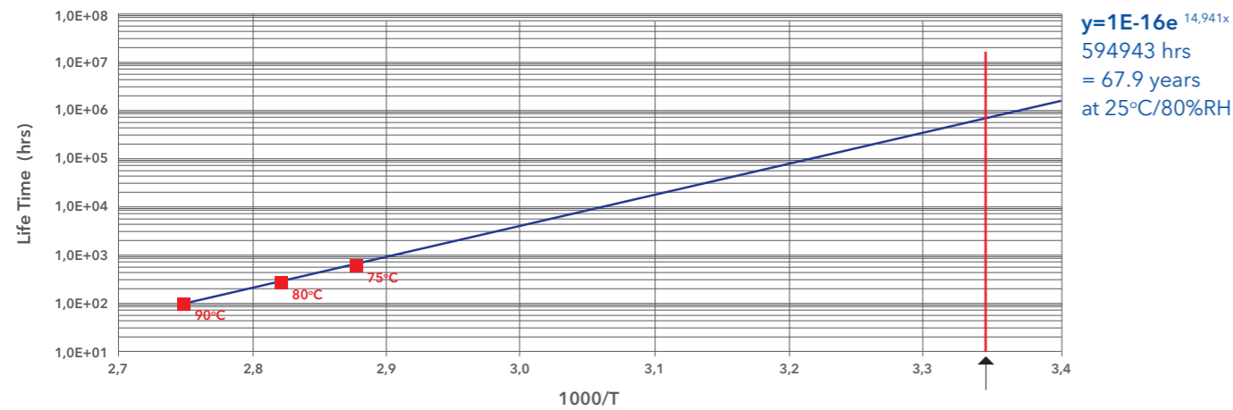
Life Estimation of MKM DVD+RDL (Life End: PI Error =280)
