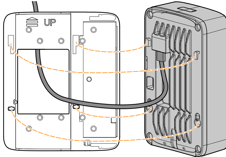
Figure 3 Secure AP-505H to Wall Mount
