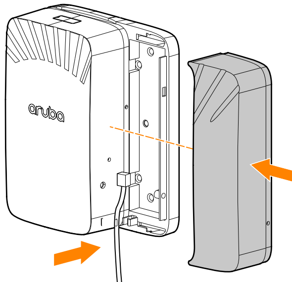
Figure 5 Attach Front Cover and Screw In Security Screw
